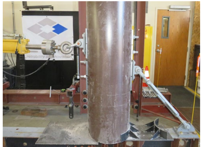
Guy Testing at EDM International
